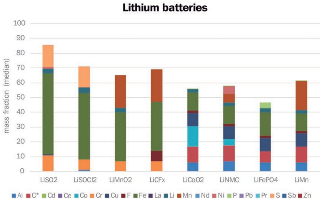
Figure 14. Composition data showing the mass fractions of specific elements in lithium-based batteries (C*: natural graphite).
