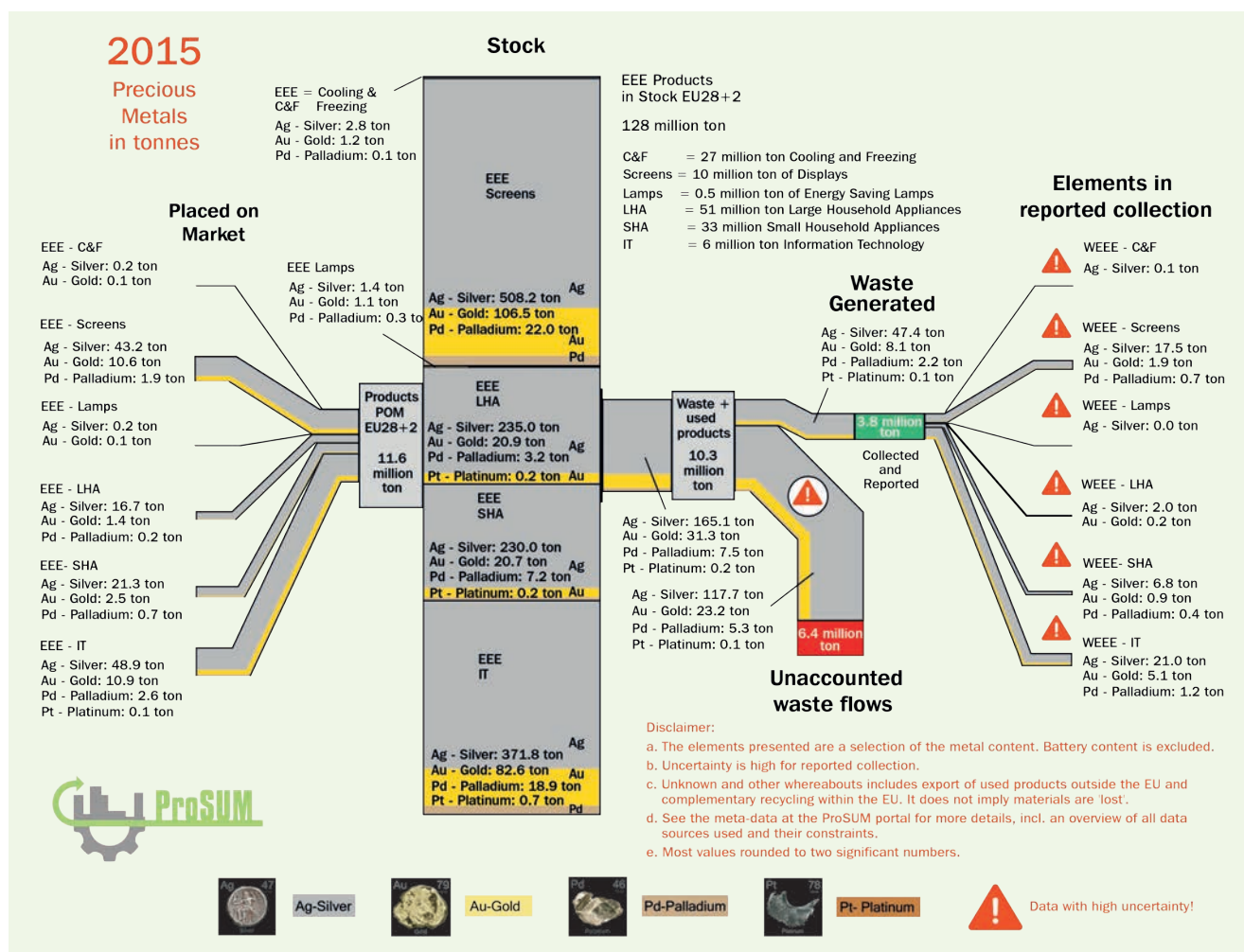
Figure 28. Stocks and Flows of precious metals in electronics in the Urban Mine, EU28+2, 2015.
